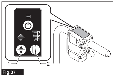
► 1. Forward/reverse button 2. Speed button
