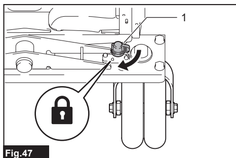
► 1. Rear wheel lock
